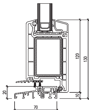
VP 70
